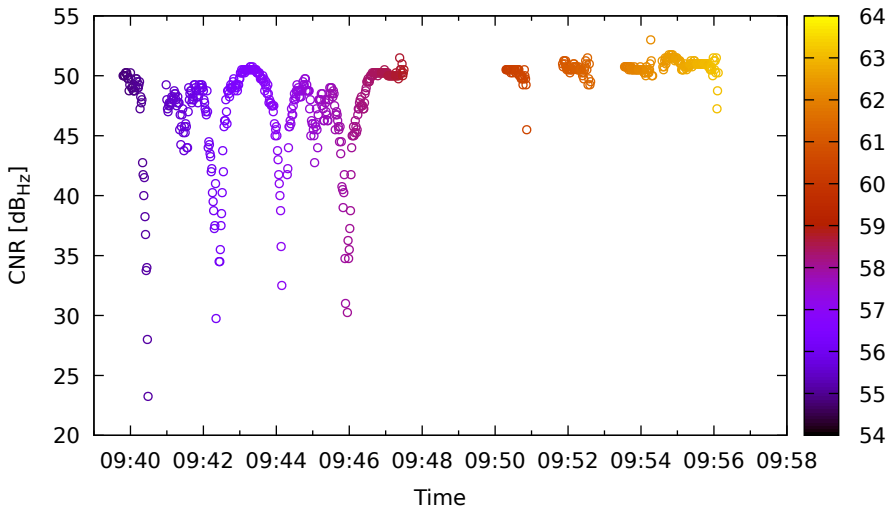
Timeline for R17 (G1) on LeicaGS18 - DOY 263
