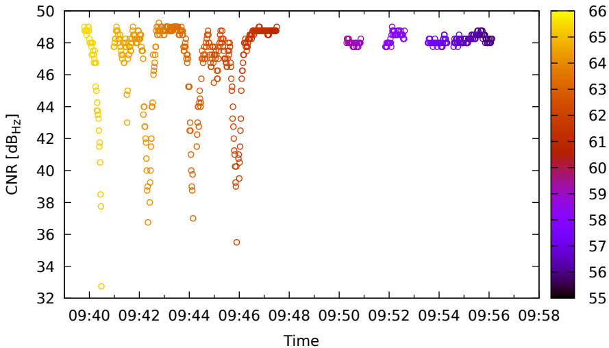
Timeline for R24 (G2) on LeicaGS18 - DOY 263
