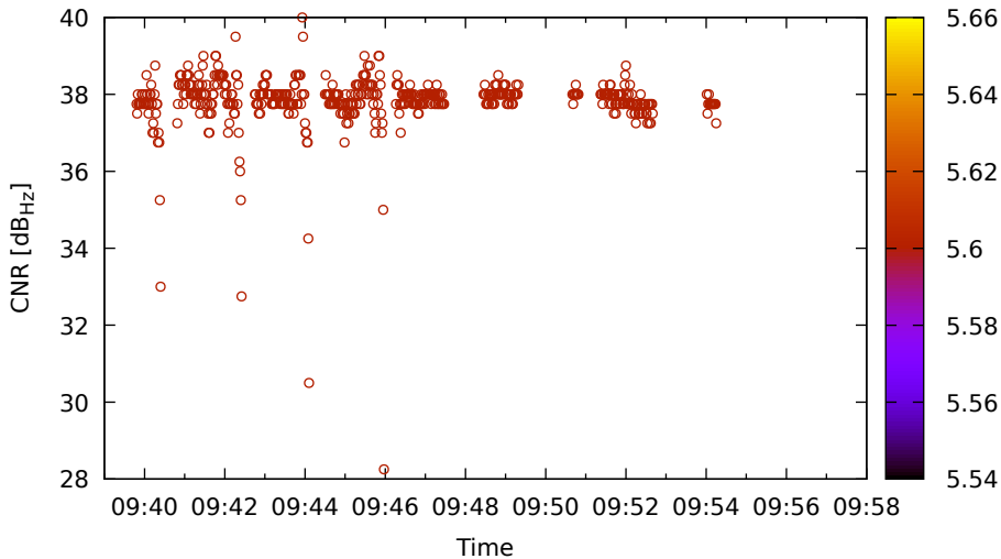
Timeline for C02 (B3) on LeicaGS18 - DOY 263
