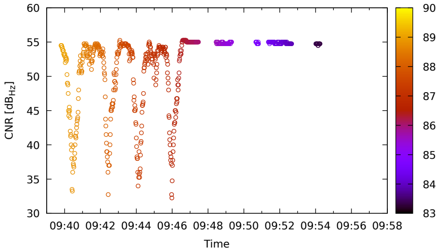
Timeline for E12 (E5) on LeicaGS18 - DOY 263
