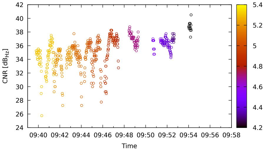
Timeline for R09 (G1) on LeicaGS18 - DOY 263
