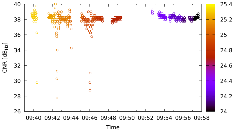
Timeline for C16 (B3) on LeicaGS18 - DOY 263
