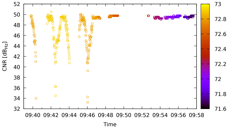
Timeline for E19 (E5a) on LeicaGS18 - DOY 263
