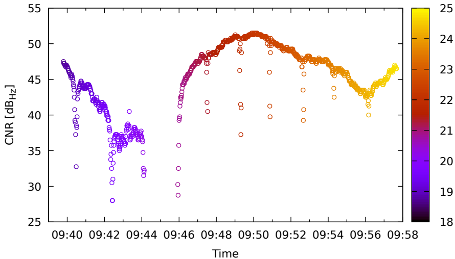
Timeline for C28 (B1) on SamsungS20 - DOY 263
