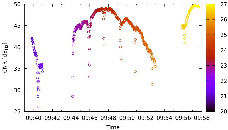
Timeline for C33 (B1) on SamsungS20 - DOY 263
