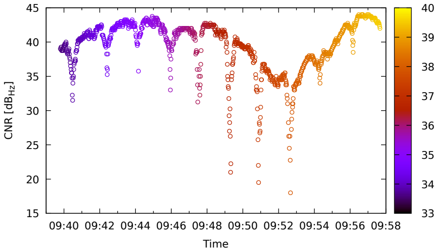
Timeline for E11 (E1) on SamsungS20 - DOY 263
