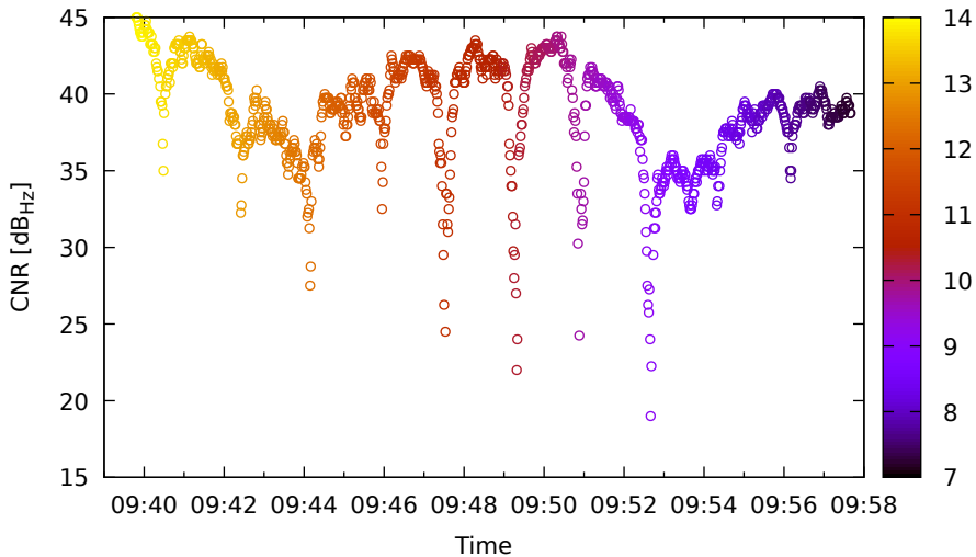
Timeline for G32 (L1) on SamsungS20 - DOY 263
