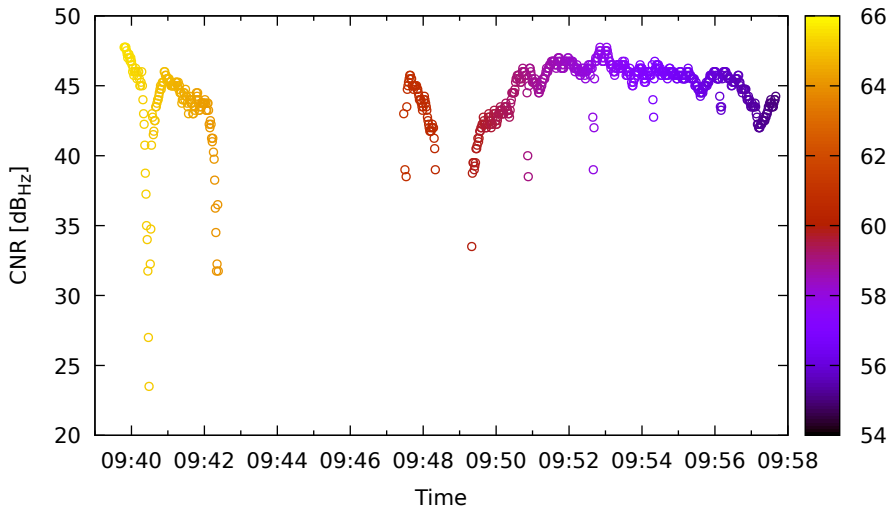
Timeline for R24 (G1) on SamsungS20 - DOY 263
