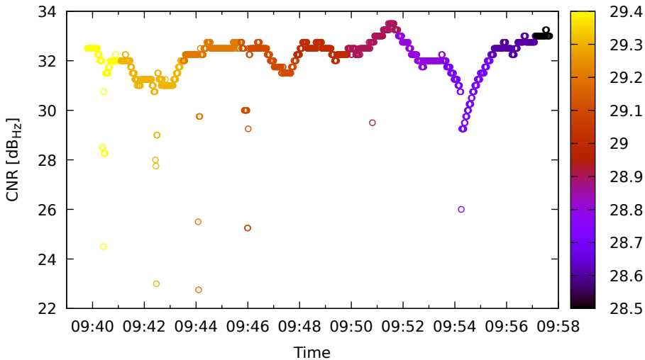
Timeline for C06 (B1) on Xiaomi11T - DOY 263
