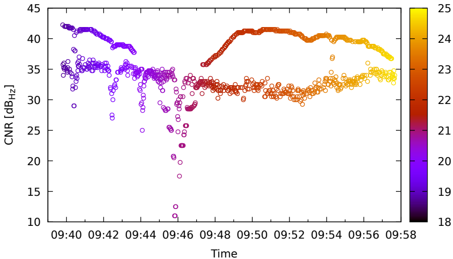
Timeline for C28 (B1) on Xiaomi11T - DOY 263
