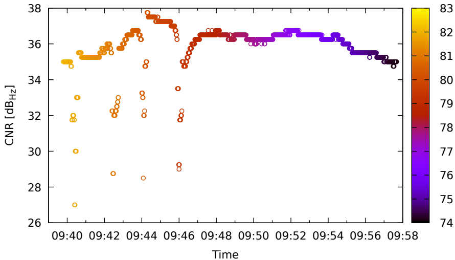
Timeline for G01 (L5) on Xiaomi11T - DOY 263
