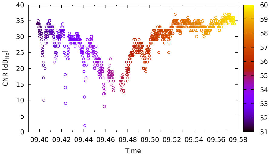
Timeline for R02 (G1) on Xiaomi11T - DOY 263
