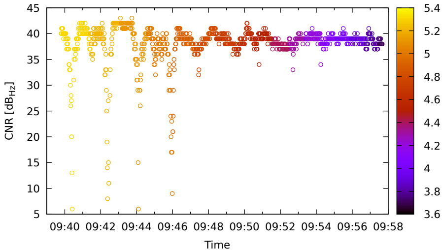
Timeline for R09 (G1) on Xiaomi11T - DOY 263
