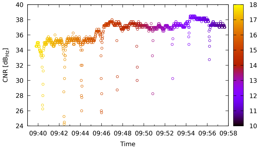
Timeline for C12 (B1) on XiaomiMi8 - DOY 263
