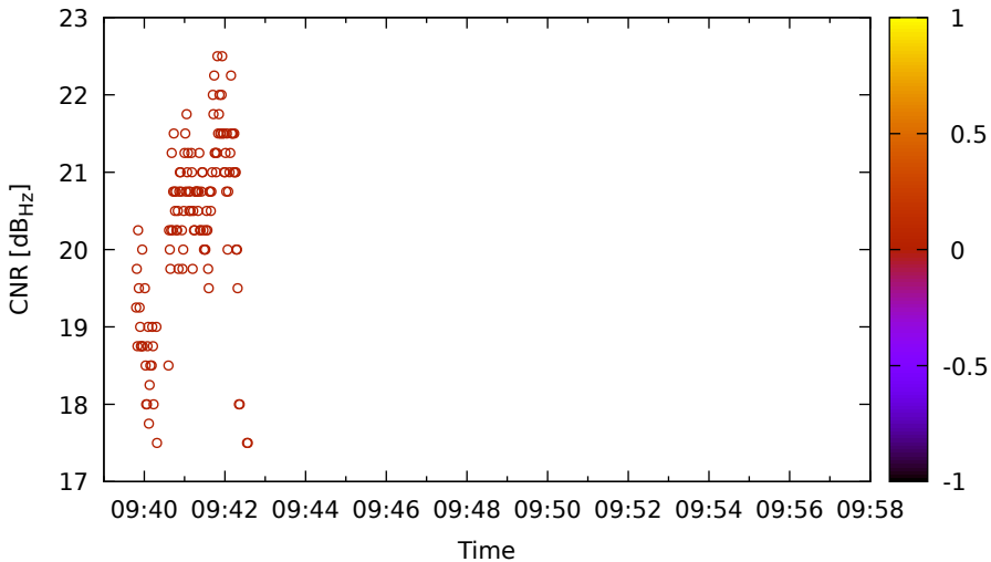
Timeline for E02 (E5a) on XiaomiMi8 - DOY 263
