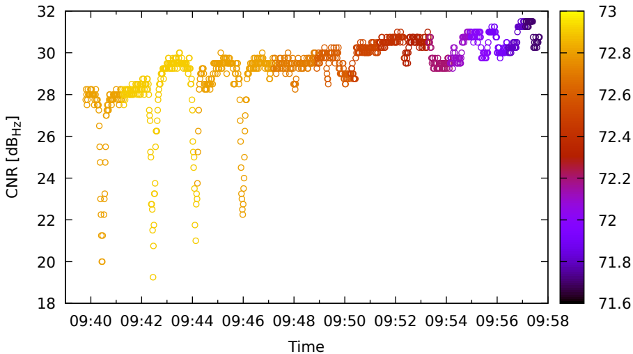
Timeline for E19 (E5a) on XiaomiMi8 - DOY 263
