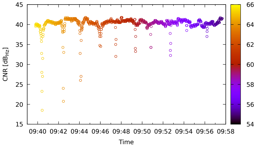
Timeline for R24 (G1) on XiaomiMi8 - DOY 263
