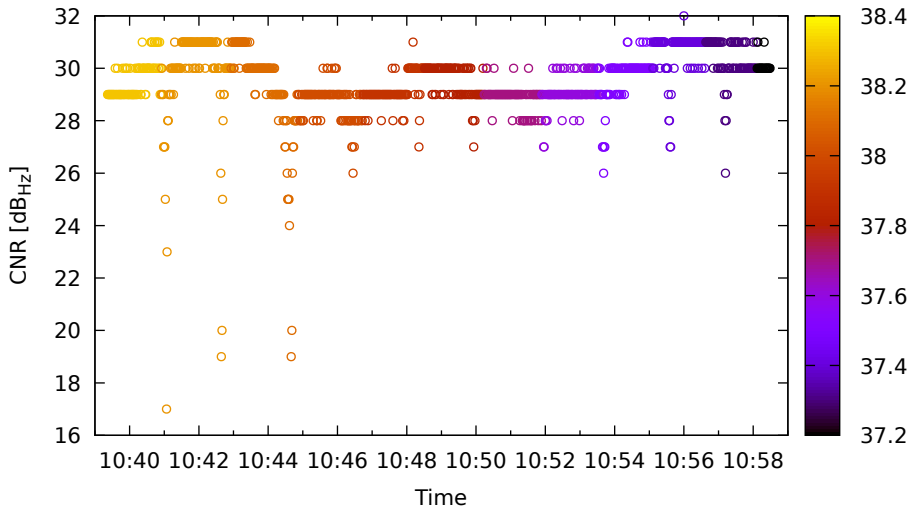
Timeline for C09 (B1) on HuaweiP40 - DOY 263
