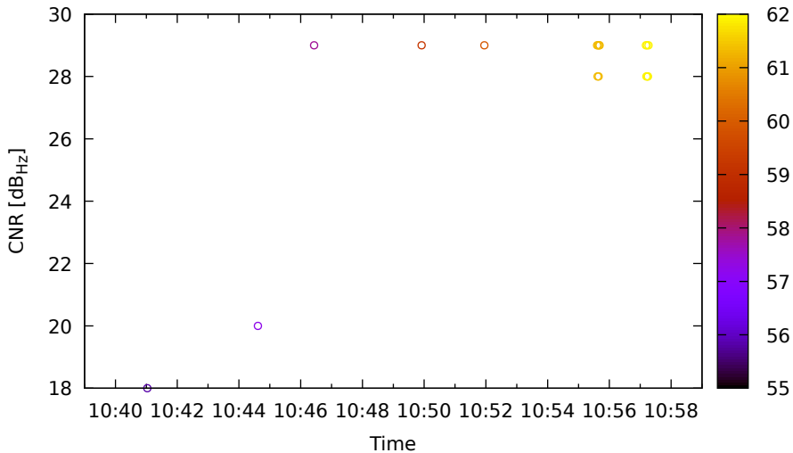
Timeline for E04 (E5a) on HuaweiP40 - DOY 263
