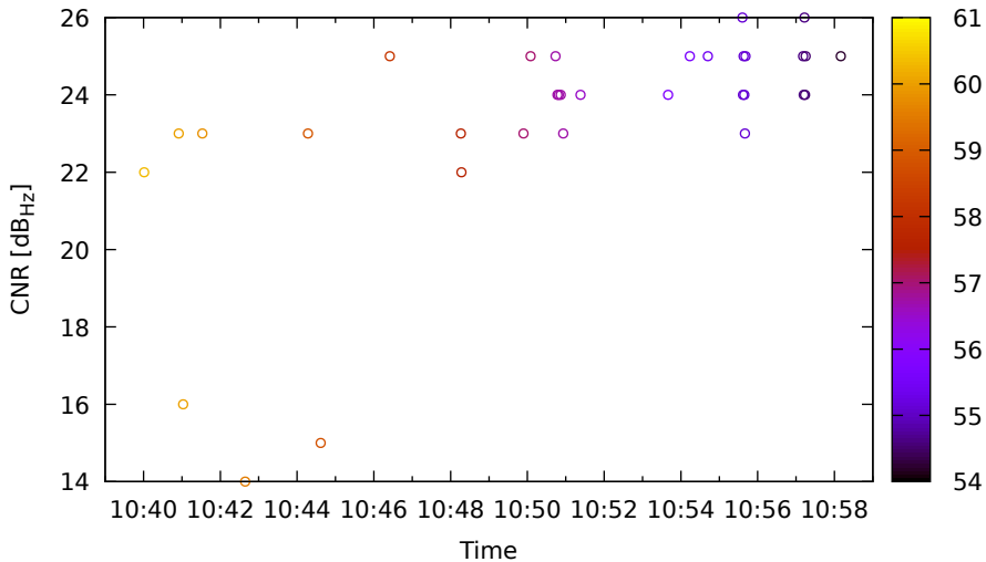
Timeline for E19 (E5a) on HuaweiP40 - DOY 263
