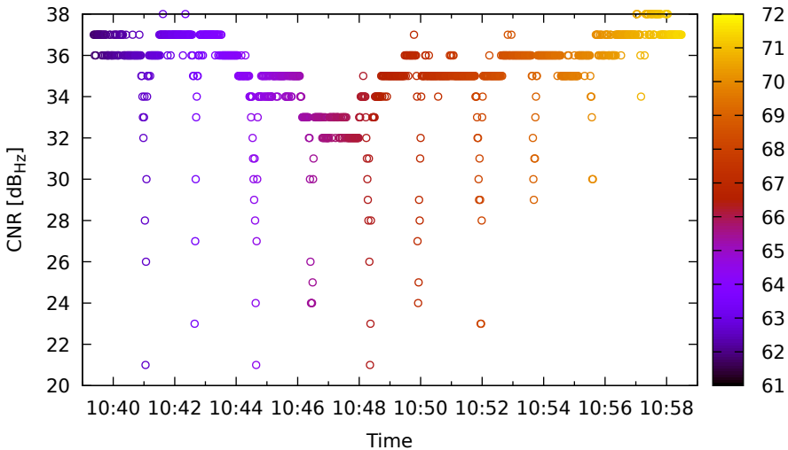
Timeline for G04 (L1) on HuaweiP40 - DOY 263
