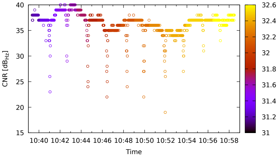
Timeline for G19 (L1) on HuaweiP40 - DOY 263
