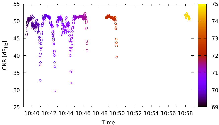
Timeline for C14 (B1) on LeicaGS18 - DOY 263
