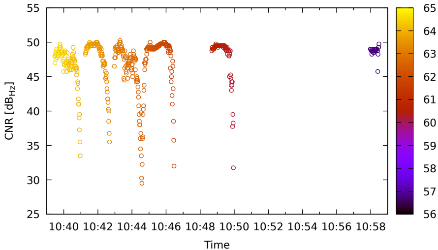
Timeline for E12 (E1) on LeicaGS18 - DOY 263
