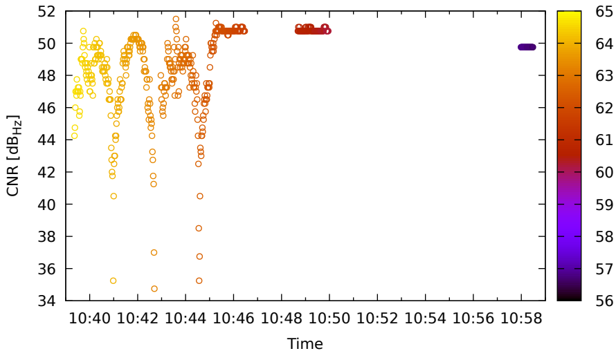
Timeline for E12 (E5a) on LeicaGS18 - DOY 263
