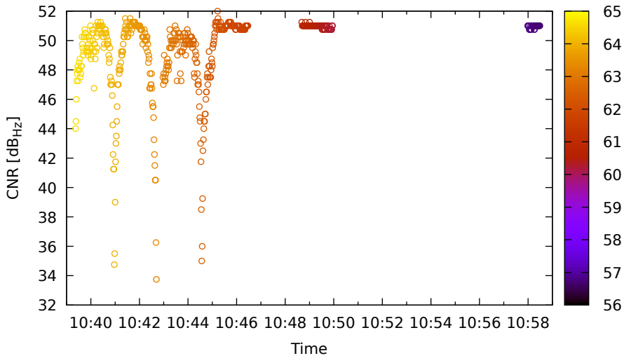
Timeline for E12 (E5b) on LeicaGS18 - DOY 263
