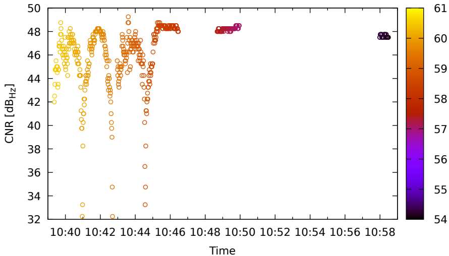
Timeline for E19 (E5a) on LeicaGS18 - DOY 263
