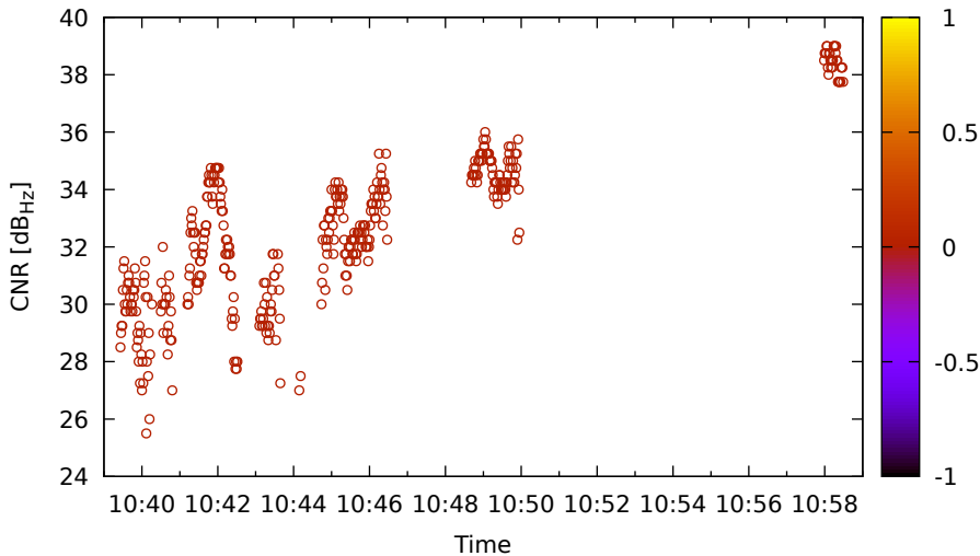
Timeline for R10 (G1) on LeicaGS18 - DOY 263
