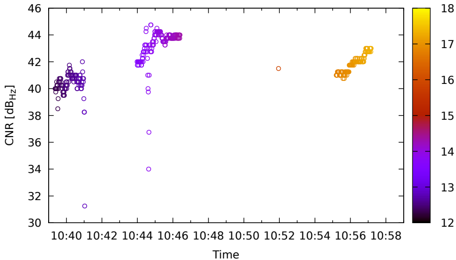
Timeline for C26 (B3) on LeicaGS18 - DOY 263
