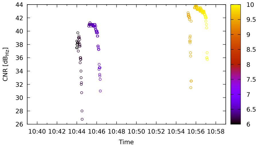
Timeline for E09 (E1) on LeicaGS18 - DOY 263
