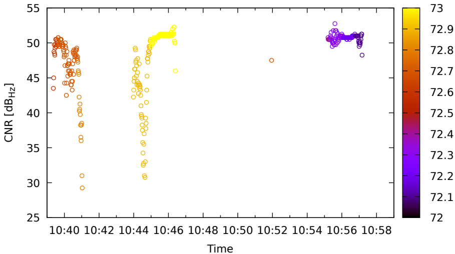
Timeline for R02 (G1) on LeicaGS18 - DOY 263
