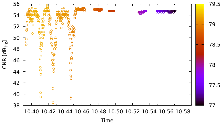
Timeline for E10 (E5b) on LeicaGS18 - DOY 263
