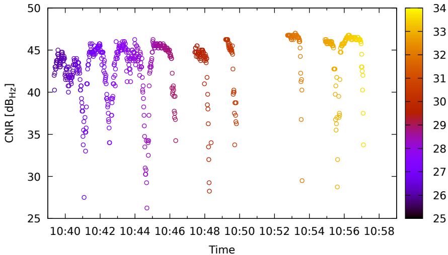
Timeline for G09 (L1) on LeicaGS18 - DOY 263
