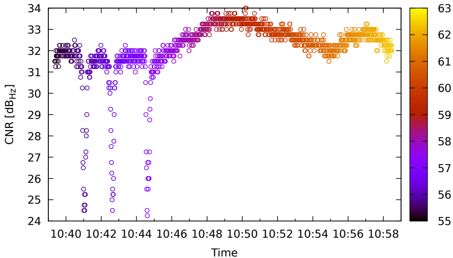
Timeline for E04 (E5a) on SamsungS20 - DOY 263
