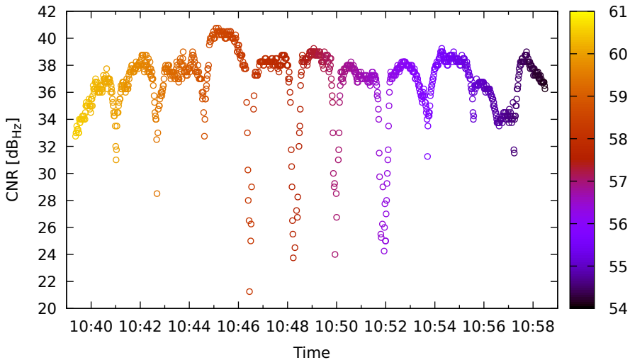
Timeline for E19 (E1) on SamsungS20 - DOY 263
