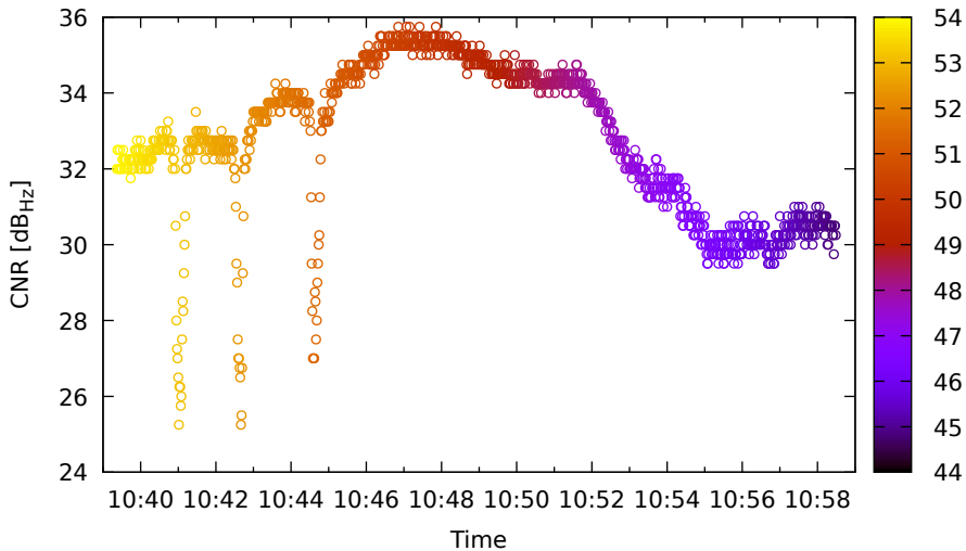
Timeline for G01 (L5) on SamsungS20 - DOY 263
