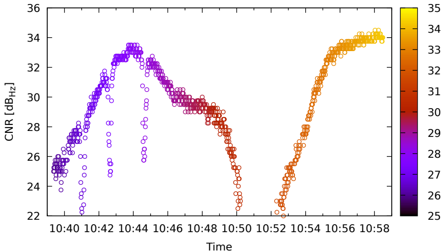
Timeline for G09 (L5) on SamsungS20 - DOY 263
