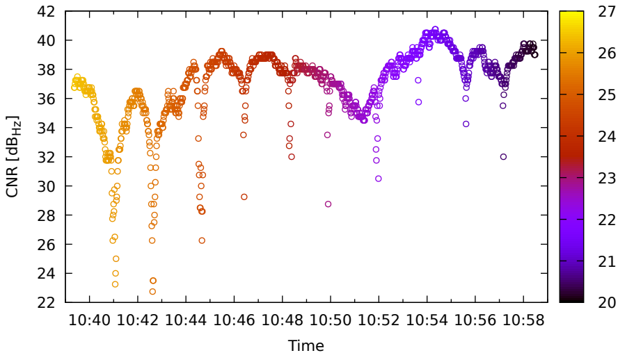
Timeline for C21 (B1) on Xiaomi11T - DOY 263
