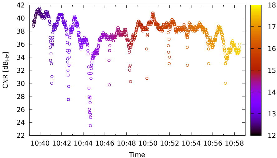
Timeline for C26 (B1) on Xiaomi11T - DOY 263
