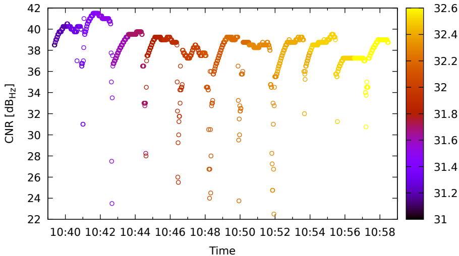
Timeline for G19 (L1) on Xiaomi11T - DOY 263
