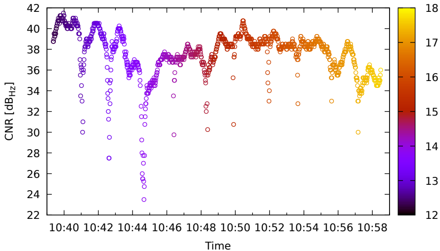
Timeline for C26 (B1) on XiaomiMi8 - DOY 263
