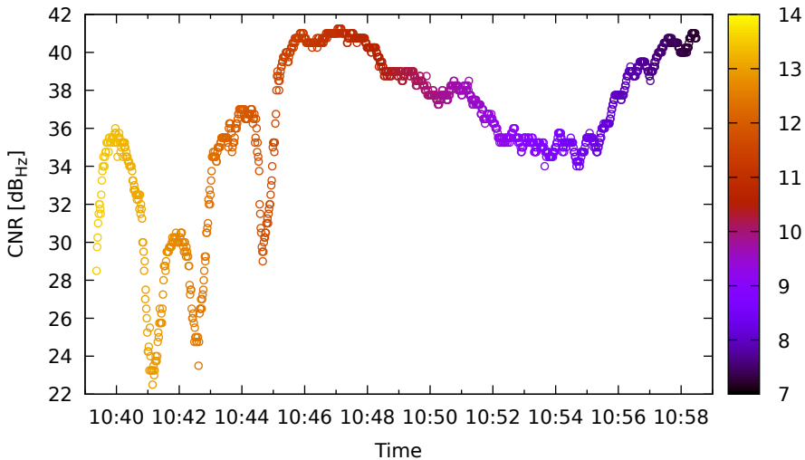
Timeline for E33 (E5a) on XiaomiMi8 - DOY 263
