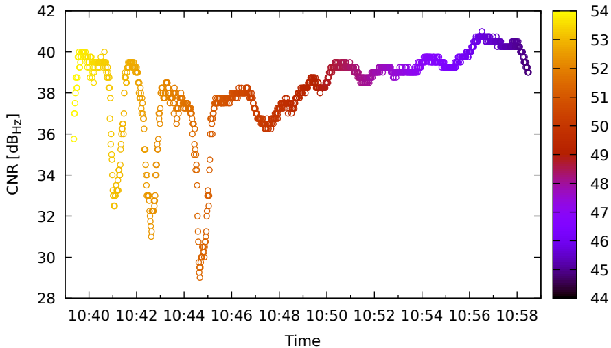
Timeline for G01 (L5) on XiaomiMi8 - DOY 263
