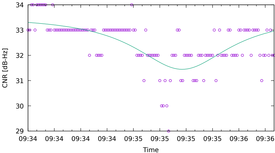
CNR fit for C06 on HuaweiP40 - drive 10 (DOY262)
