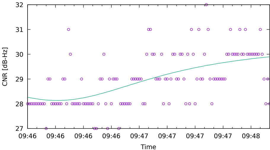
CNR fit for C09 on HuaweiP40 - drive 16 (DOY262)
