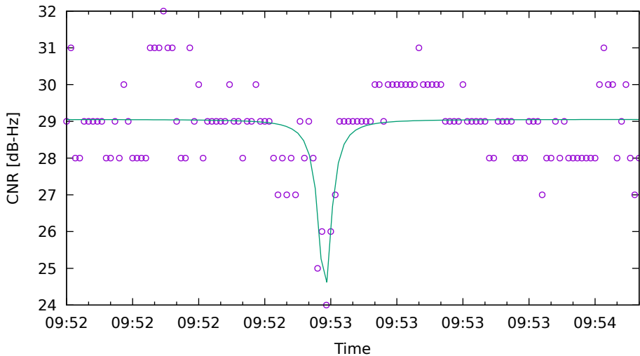
CNR fit for C09 on HuaweiP40 - drive 19 (DOY262)
